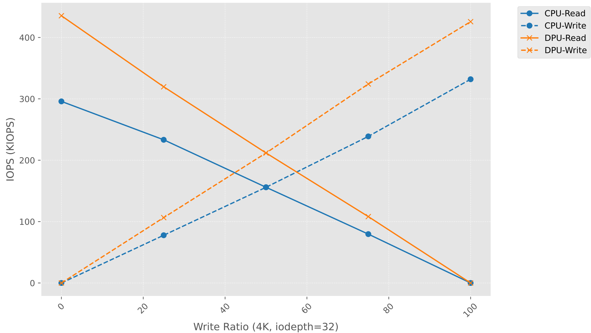
IOPS vs Write Ratio (4K, iodepth=32)
